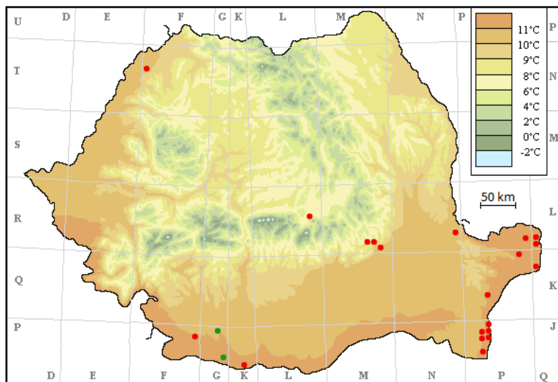
Fig. 5. Distribution of the species Polypogon monspeliensis in Romania, correlated with the average annual temperature.
