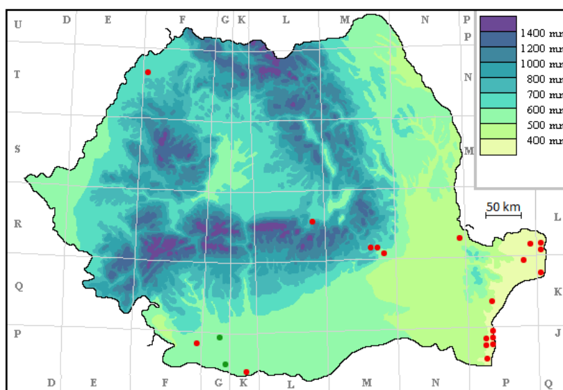
Fig. 6. Distribution of the species Polypogon monspeliensis in Romania, correlated with the average annual precipitation.
